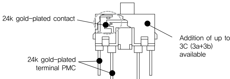
Contact block (1a+1b), product name: FCB
