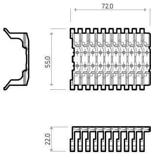
KTB3-01010C
