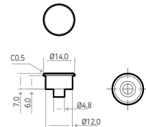
KTB1-CAP
