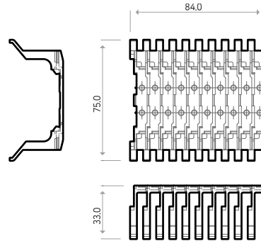
KTB3-01510C
