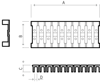
KTB1-C Type Safety Cover
